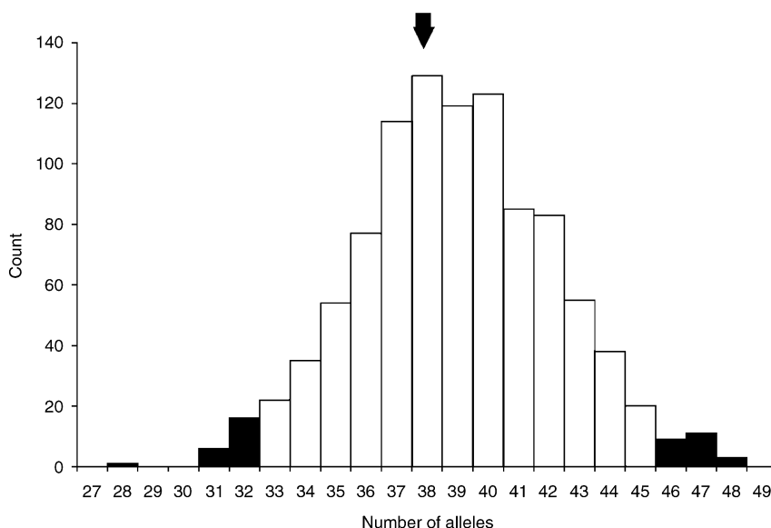
Fig. 4 Expected distribution for the number of microsatellite alleles in seven individuals randomly drawn from the North American population (results based on 1000 random samples). The arrow indicates the number of alleles found in the feral population in Europe. The 95% confidence interval (white colour) was determined by calculating the 0.025 and 0.975 percentiles (black colour).
