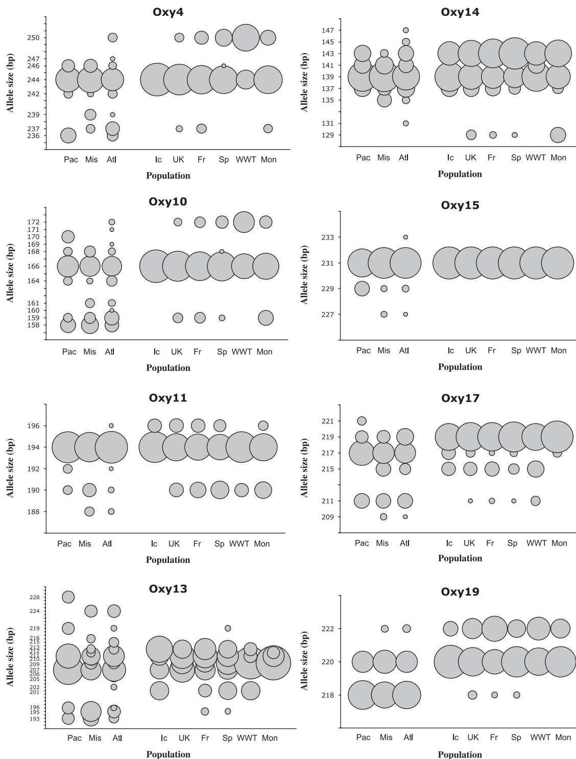
Fig. 3 Allelic frequencies for eight microsatellite loci in ruddy ducks in relation to geographical location. (Pac, Pacific; Mis, Mississippi; Atl, Atlantic; Ic, Iceland; UK, United Kingdom; Fr, France; Sp, Spain; WWT, Wildfowl and Wetlands Trust; Mon, Monmouth.) Three additional loci (Oxy1, Oxy3, Oxy6) showed lower allelic diversity in both populations. These loci had 3 and 3 alleles; 2 and 1 alleles; and 2 and 2 alleles in North America and Europe, respectively. The area of each circle is proportional to the relative frequency of each allele.
